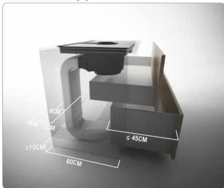
NIKOLATESLA VERSION EXTRACTION STANDARD NikolaTesla standaard afzuiging
